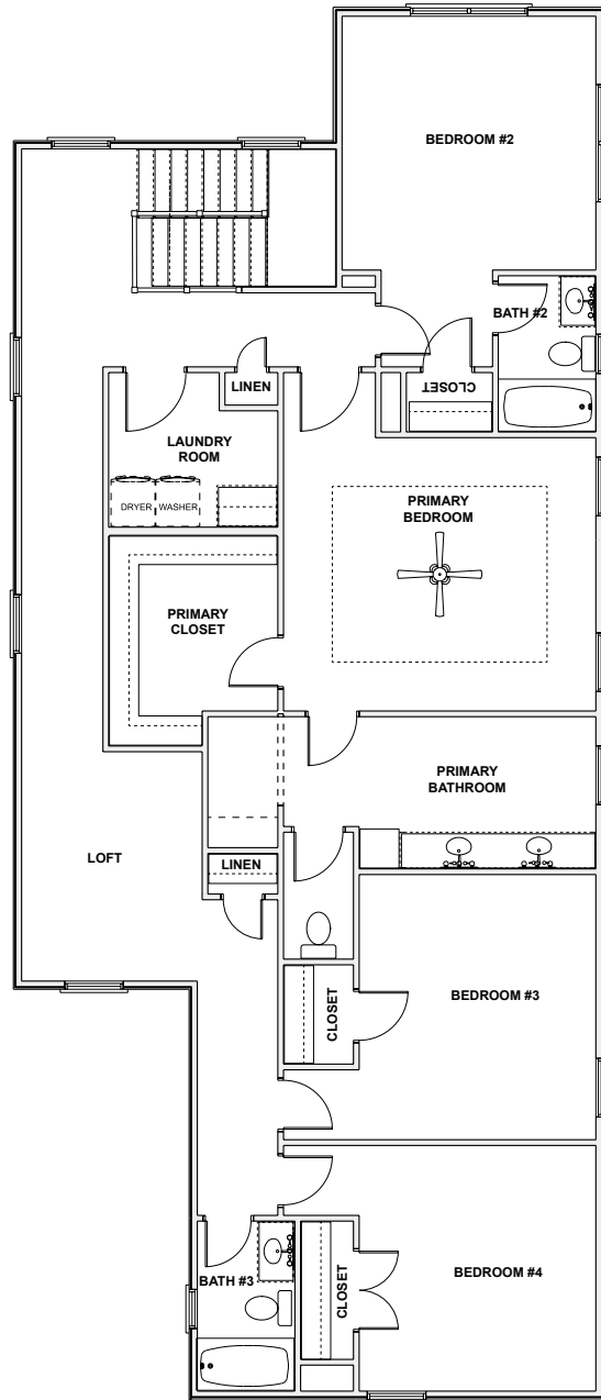
SECOND FLOOR
